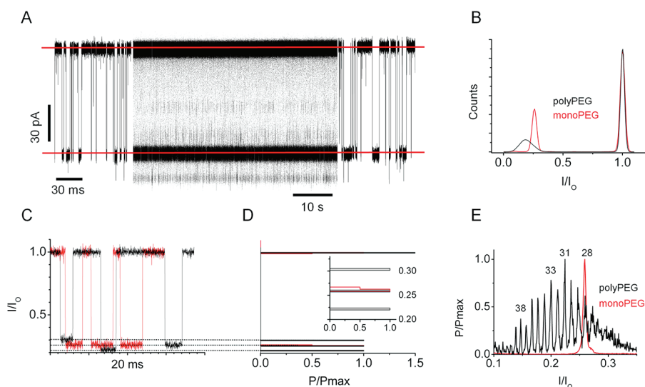
Figure 2. Current traces and histograms derived from recordings of \alpha HL pores blocked by monoPEG-28 and polyPEG-1500 on one MEC ( \varnothing 16 \mu m) of a 16-cavity chip with a SCA (Axopatch 200B) filtered at 20 kHz and digitized at 200 kHz. The MEC was held at V_h = +40 mV with respect to the cis -side; 4 M KCl. (A) 60 s trace of one \alpha HL pore blocked by monoPEG. The initial and last 100 ms are shown on an expanded time scale. Note the stability of the current detected with one MEC over time (see reference lines). (B) All-points histogram of the trace shown in (A). Different distributions are obtained for monoPEG-28 (red) and polyPEG-1500 (black). Both distributions appear unimodal. (C) Three blockage events from experiments with monoPEG (red) and polyPEG (black). Note that polyPEG-induced blocks visit distinct levels. (D) Event-averaged histogram of the traces shown in (C). Probability P is normalized to the highest peak. Distinct levels can be clearly distinguished (polyPEG at I/I_o = 0.22 , 0.26, and 0.30; monoPEG at I/I_o = 0.26 ). (E) Event-averaged histograms for 6.408 (polyPEG, black) or 19.318 (monoPEG, red) events (open state not shown). The multimodal distribution of polyPEG can be clearly distinguished from the monoPEG distribution. The different peaks can be assigned to the length of the particular PEG molecules of the polyPEG solution. Blockages of molecules with higher molecular weight result in lower ratios of I/I_o . With reference to the peak of the monoPEG-28-histogram (red) the peaks in the polyPEG distribution can be assigned a specific polymer size by increments or decrements of one repeat unit. 28
